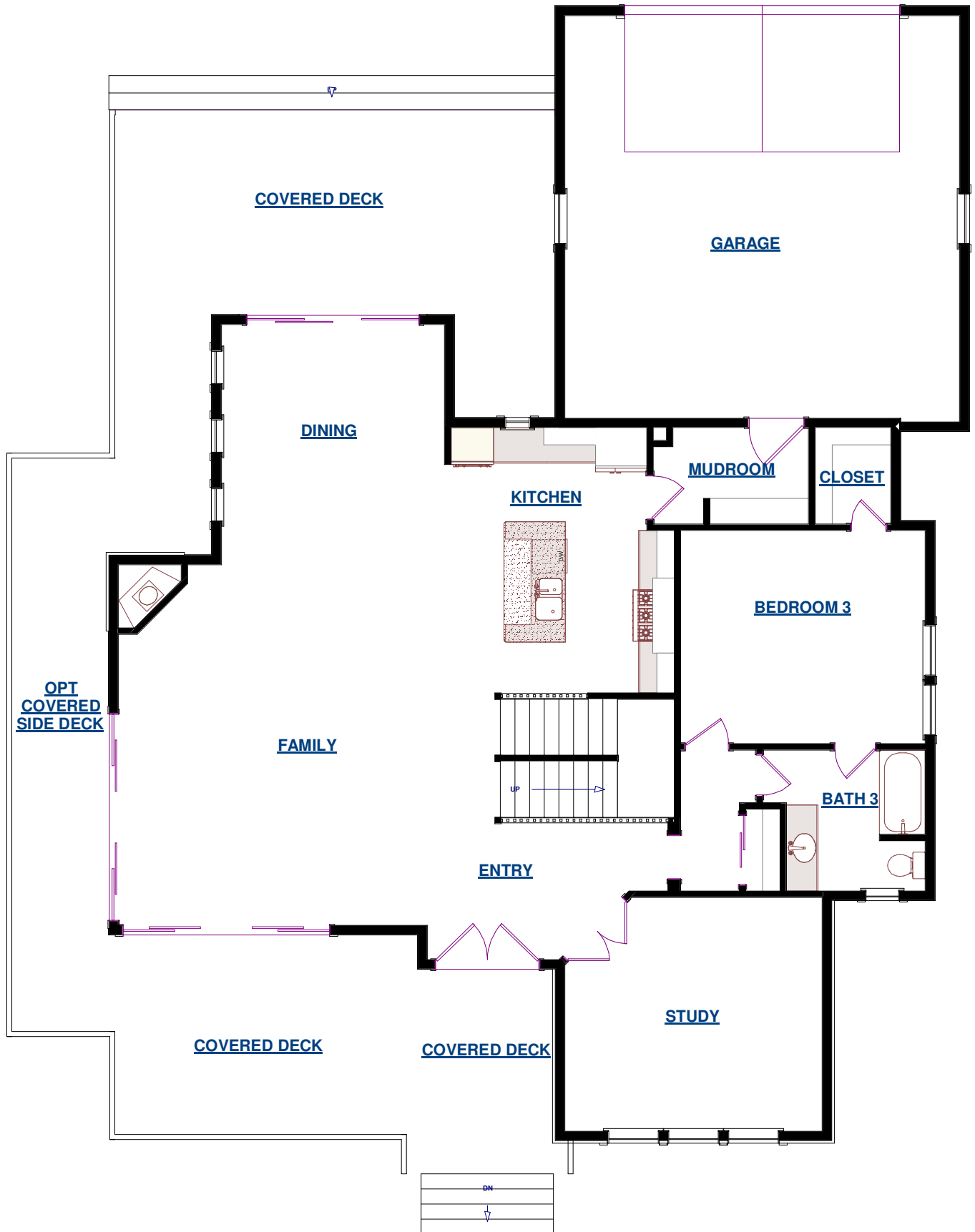
MAIN LEVEL FLOOR PLAN 1589 sq ft
